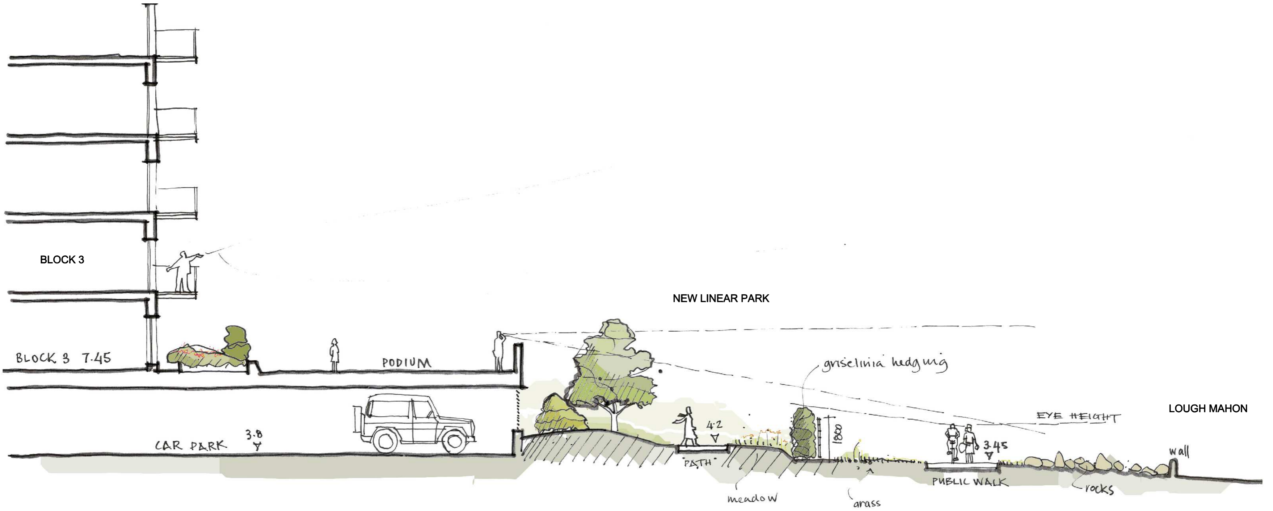
Section through Block 3 and the Interface with Mahon Walk illustrating the relationship between the apartments, podium deck over car park, linear park and Lough Mahon Walk
